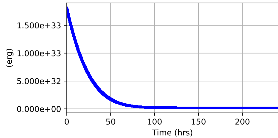
Total Thermal Energy
