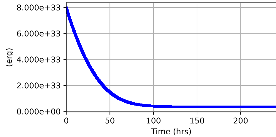
Total Kinetic Energy
