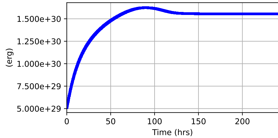
Total Magnetic Energy
