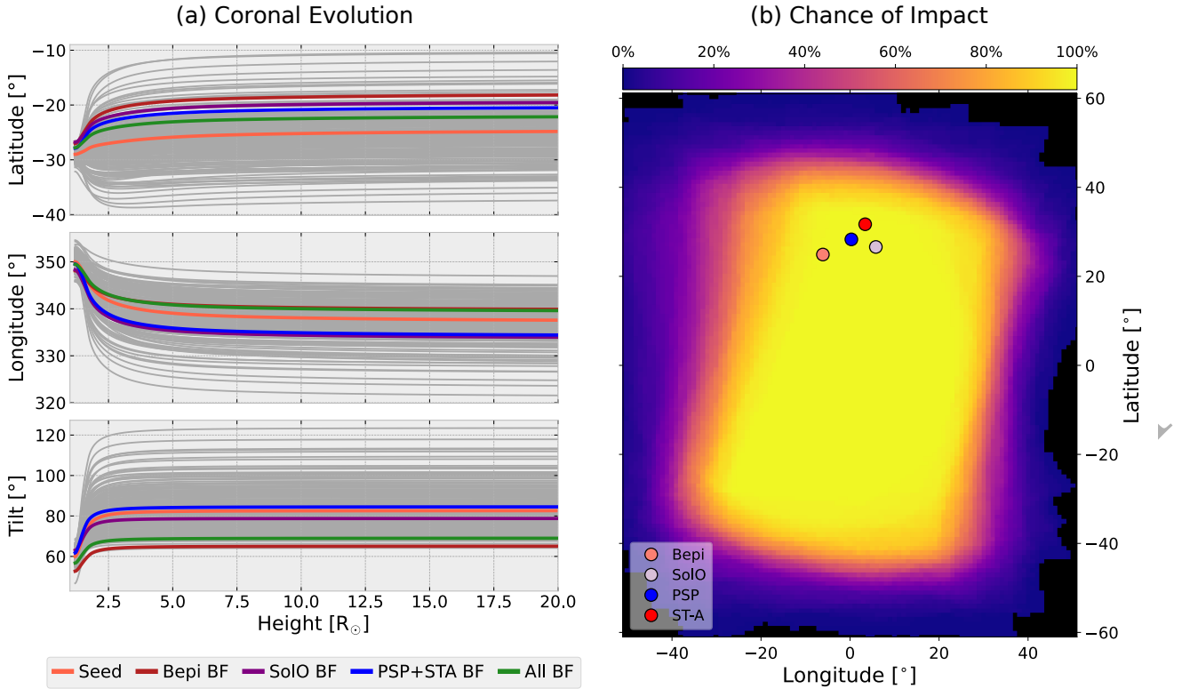
Figure 8. Overview of the (a) coronal and (b) heliospheric evolution of the (200-member) ensemble CME run modelled with OSPREI. (a) ForeCAT deflections and rotations up to 20 R_{\odot} . The seed run as well as the various best-fit runs are highlighted in different colours, whilst the remaining ensemble members are shown in grey. (b) Radial slice of the CME angular extent at the time of impact at PSP, shown as a heat map representing the chance of impact at a given latitude–longitude coordinate across the ensemble. The superposed circles mark the projected positions of the four spacecraft at their respective observed CME arrival times (i.e., the times shown in Table 1). The figure is displayed in the frame centred at the CME nose of the seed run.
