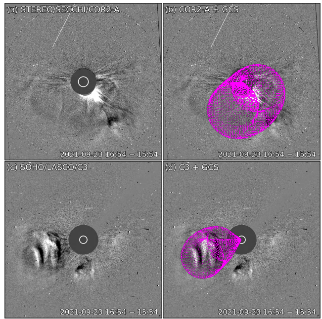
Figure 3. The faint 23 September 2021 CME observed in WL imagery from (top) STEREO-A and (bottom) SOHO. The left panels show plain coronagraph difference images, whilst the right panels display the same data with the GCS wireframe overlaid.
