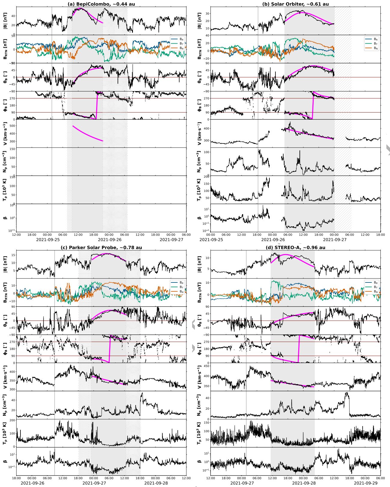
Figure 4. In-situ measurements of the 23 September 2021 CME at (a) Bepi, (b) SoLo, (c) PSP, and (d) STEREO-A. Each plot shows, from top to bottom: magnetic field magnitude, magnetic field components in Radial–Tangential–Normal (RTN) coordinates, latitudinal and longitudinal angles of the magnetic field, solar wind bulk speed, proton density and temperature, and plasma beta. Interplanetary shocks arrivals are marked with vertical areas, whilst CME ejecta regions are highlighted with shading—the core flux rope in solid colour and other ejecta boundaries in dotted (Bepi and PSP) or hatched (SoLo) markings—see the main text for details. The magenta curves show flux rope fitting results using the EFF model. The heliocentric distances reported on top of each plot refer to the respective shock arrival time at each spacecraft (see also Table 1). Note that each panel displays 2.75 days of data.
