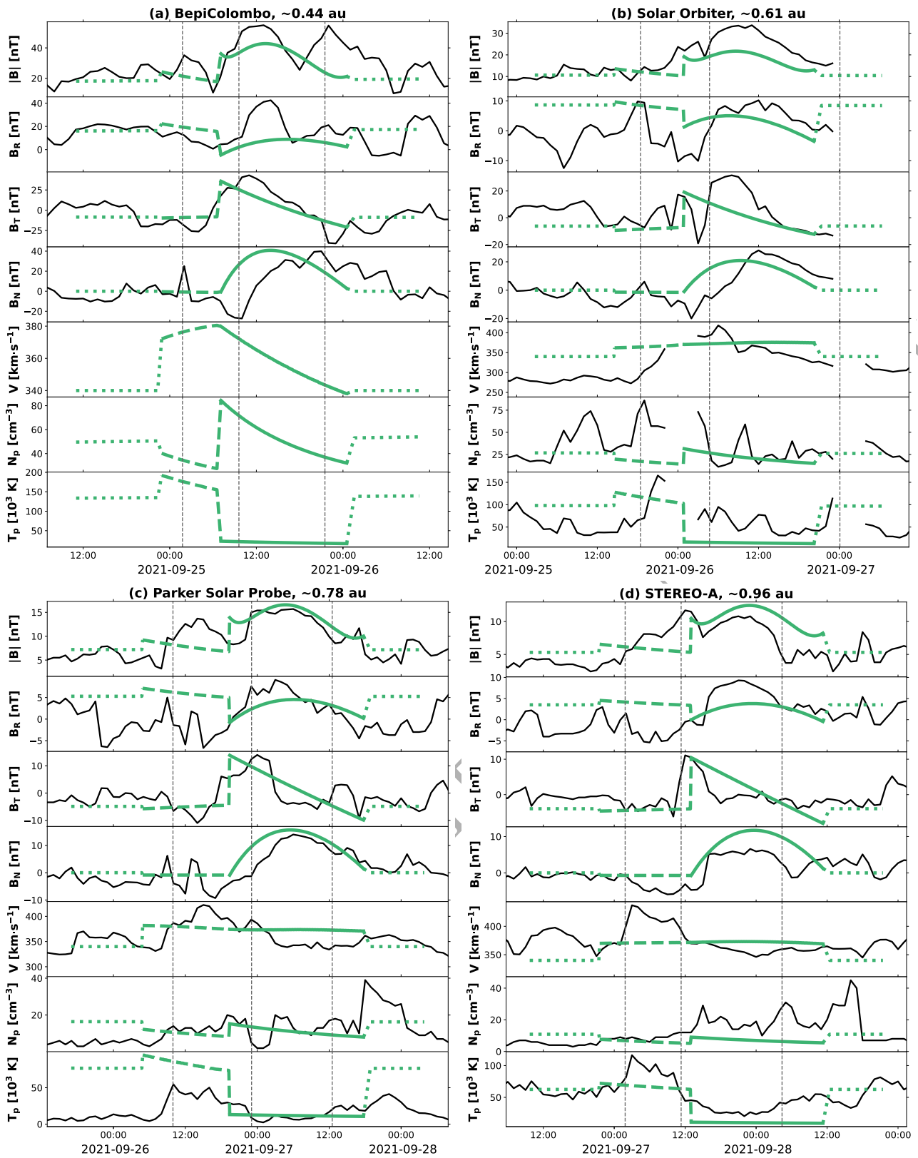
Figure 11. Overview of the OSPREI seed simulation run results with latitudinally-mirrored (with respect to the CME nose) spacecraft crossings shown against in-situ measurements of the 23 September 2021 CME at (a) Bepi, (b) SOLO, (c) PSP, and (d) STEREO-A. All panels and parameters are shown in the same format as Figure 7.
