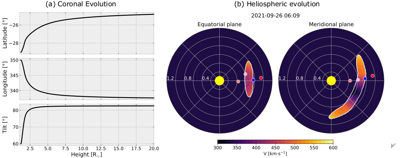
Figure 6. Overview of the (a) coronal and (b) heliospheric evolution of the CME modelled as the seed run for OSPREI. (a) ForeCAT deflections and rotations up to 20 R_{\odot} . (b) Snapshot of the CME evolution in interplanetary space as seen from (left) the equatorial and (right) the nose-centred meridional planes. The quantity shown is the solar wind bulk speed, and the four circles represent the positions of the four spacecraft (by increasing distance from the Sun, Bepi, SoLo, PSP, and STEREO-A) projected onto the respective planes.
