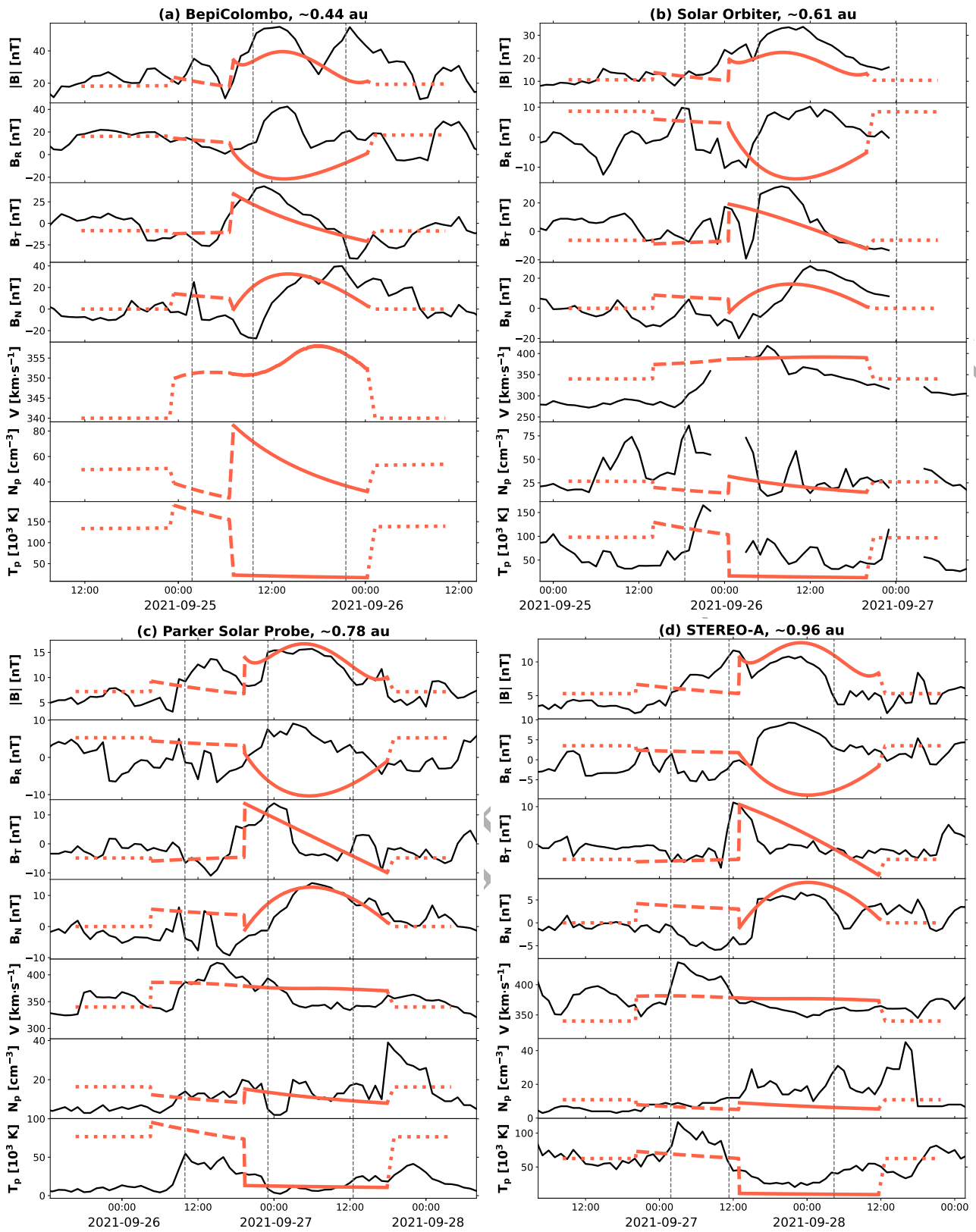
Figure 7. Overview of the OSPREI seed simulation run results shown against in-situ measurements of the 23 September 2021 CME at (a) Bepi, (b) SoLo, (c) PSP, and (d) STEREO-A. Each plot shows, from top to bottom: magnetic field magnitude, magnetic field Cartesian components in RTN coordinates, solar wind bulk speed, as well as proton density and temperature. The spacecraft data are displayed in black, whilst the OSPREI synthetic profiles are shown in orange for (dotted) background wind, (dashed) sheath region, and (solid) CME ejecta intervals. The dashed vertical lines mark (leftmost) the shock arrival and (remaining two) the flux rope boundaries as observed by each spacecraft.
